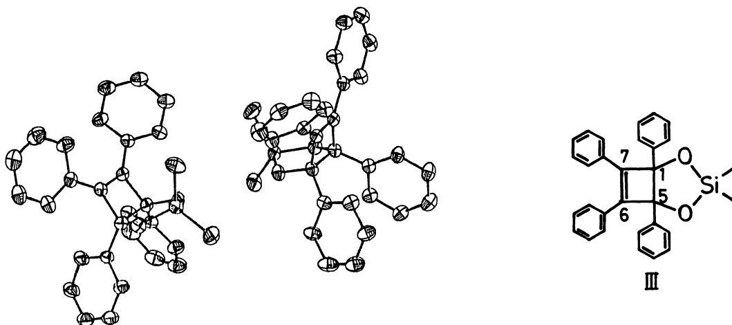
Figure 1. ORTEP drawing of the molecular structure of III which was determined by X-ray diffraction method. Crystal Data: a=13.822(2) , b=9.892(1) , c=21.701(2)\text{\AA} , \alpha=79.46(1) , \beta=119.10(1) , \gamma=107.83(1)^\circ , space group= P\bar{1} ( Z=4 ). The R value was reduced to 0.09 for 6837 observed reflections by anisotropic non-hydrogen atoms refinements. This figure shows two molecules in the unit cell and their molecular geometries are essentially the same except for the torsion of phenyl group. Selected bond lengths averaged among equivalent bonds over two independent molecules are: Si-O= 1.658(5) , C(1)-C(5)= 1.60_2 , C(1)-C(7)= 1.52_7 , C(6)-C(7)= 1.35_1\text{\AA} .
